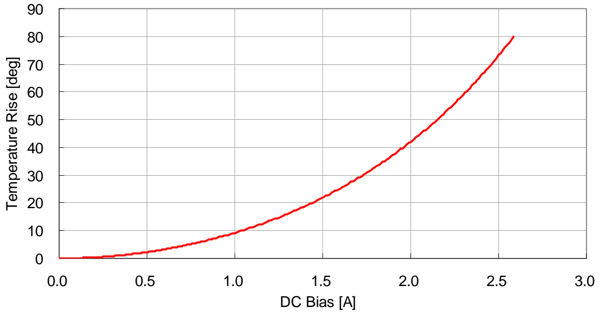
VLS252015 1R5N1R4
