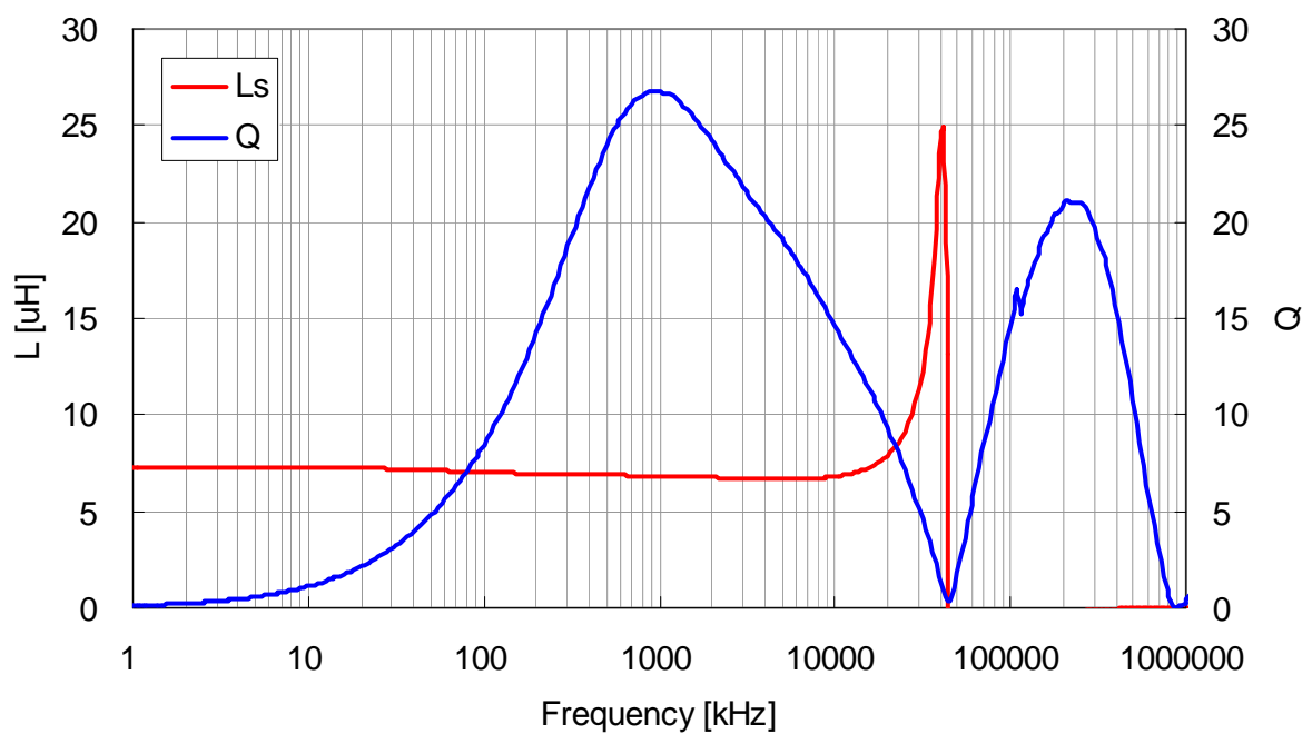
VLS252015 6R8MR73
